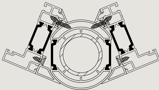
Variable Baypole
