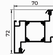
WQ19 WIDE 'Z' MULLION
