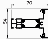
WQ10 SLIM 'T' MULLION WITH SCREW PORTS
