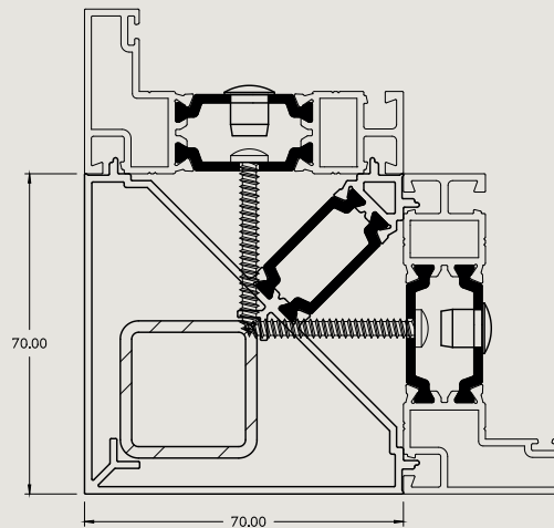
90 degree Baypole
