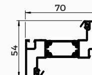
WQ13 SLIM 'Z' MULLION
