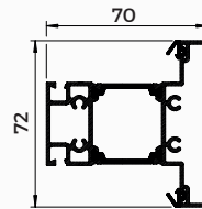
WQ16 WIDE 'T' MULLION WITH SCREW PORTS
