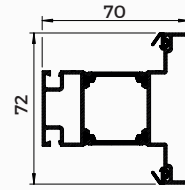
WQ18 WIDE 'T' MULLION
