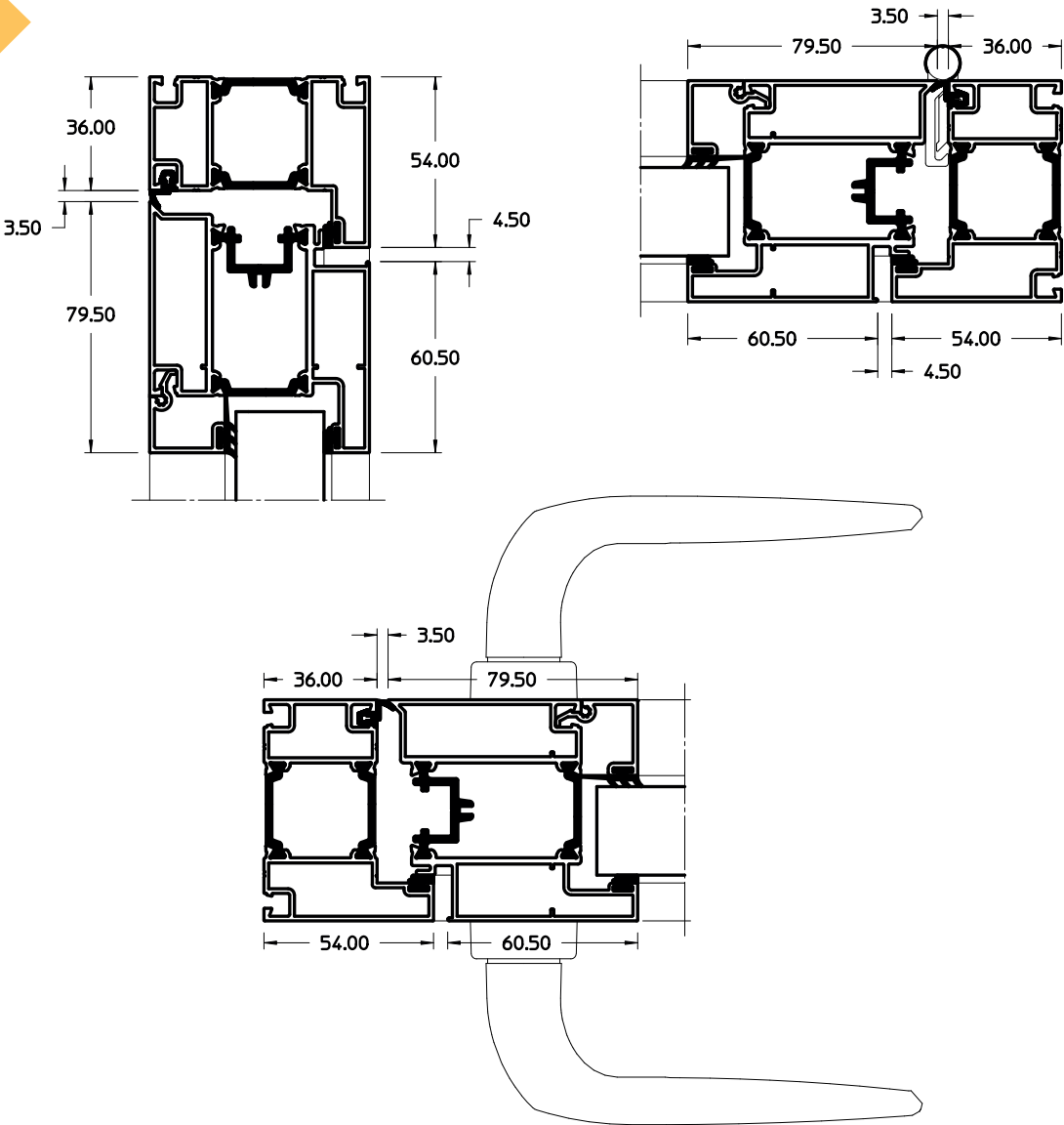
Single Door
