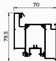
WQ40 DOOR 'Z' SASH
