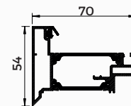
WQ32 FULLY FLUSH SASH
