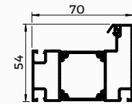
WQ02 MEDIUM OUTER FRAME
